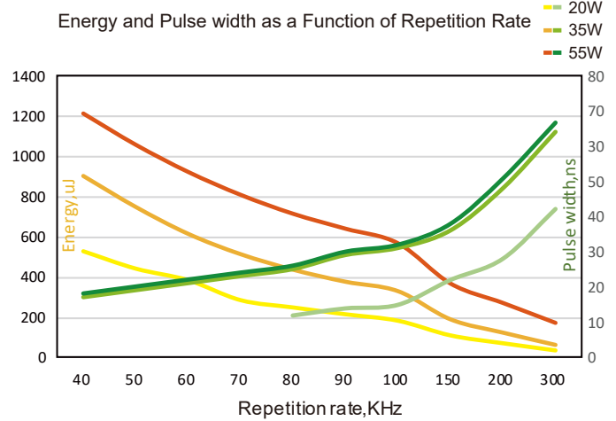
Typical Performance AONano Precision 532-20W/35W/55W
