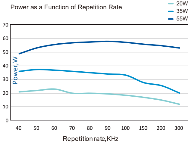
Typical Performance AONano Precision 532-20W/35W/55W
